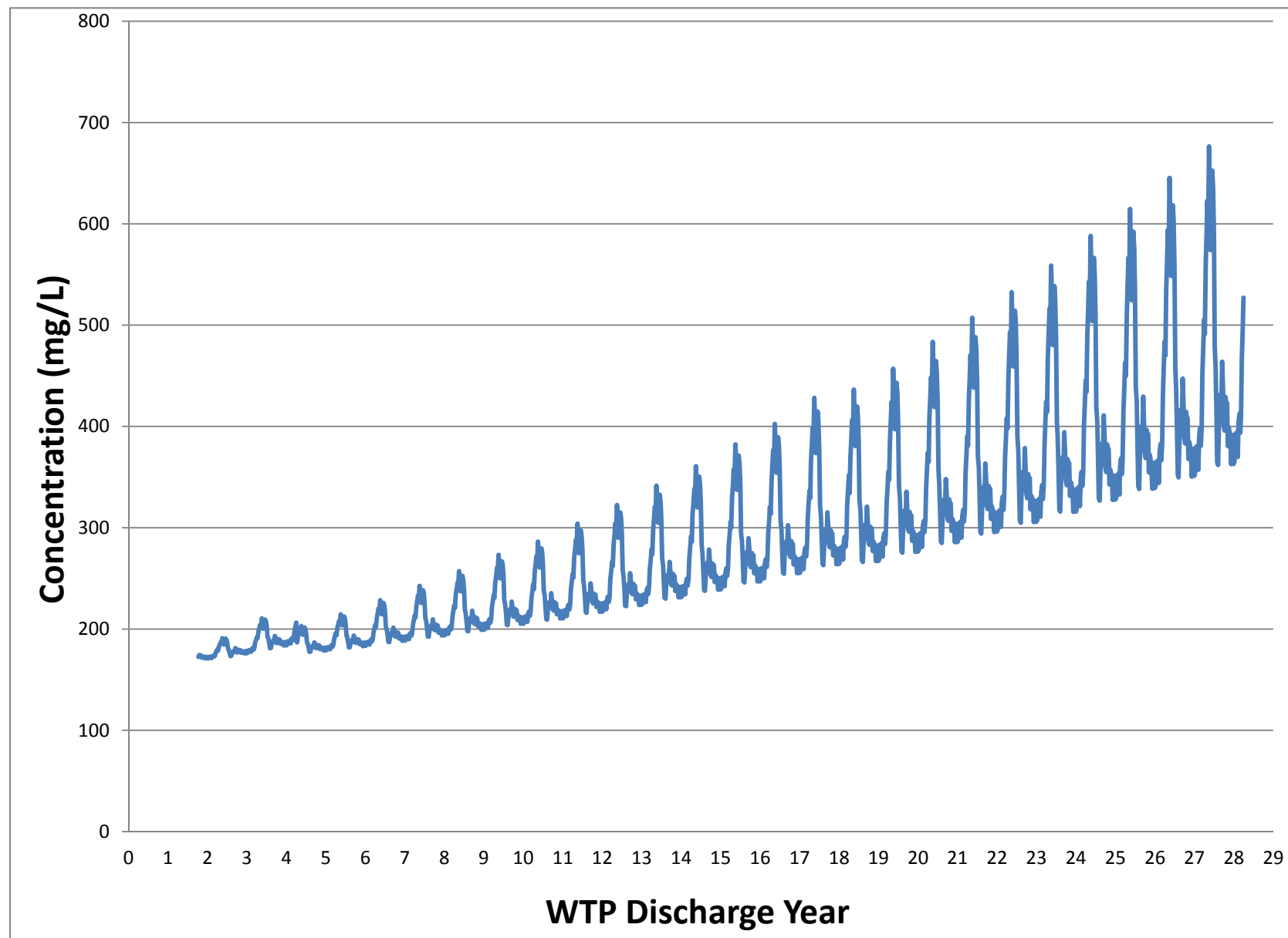
Figure 6: Predicted TDS Concentration in the SRS, Average Flow Conditions
