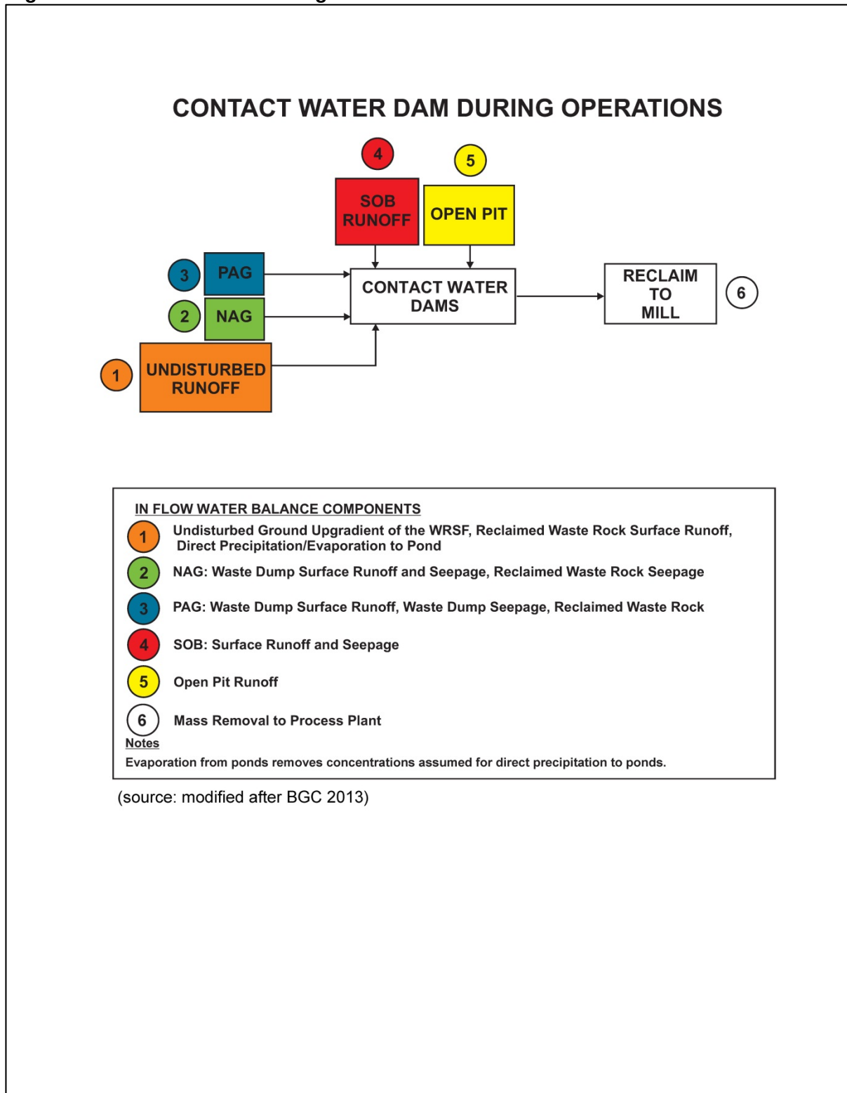
Figure 4: Areas Contributing Flow to the Lower CWD
