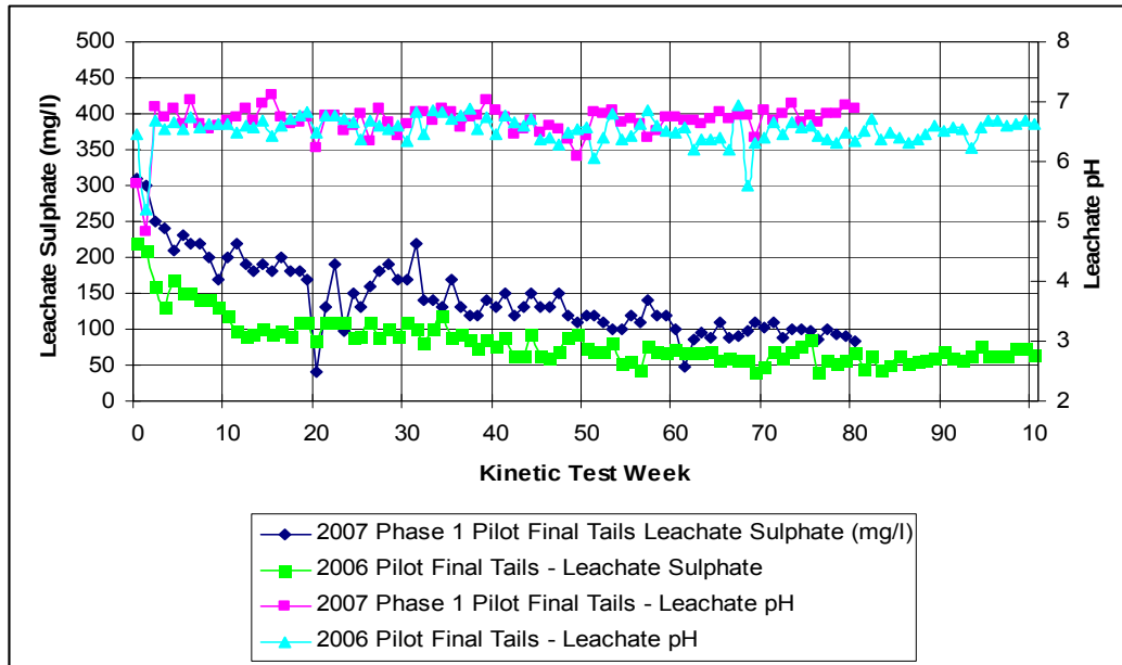
Figure C-6: Kinetic Cell Testing Profiles (pH, sulfate) of Two Final Tailings Samples
