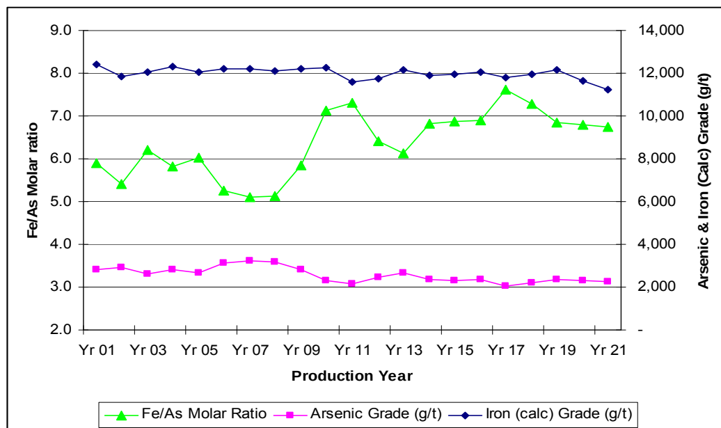
Figure C-8: Production Plan for Arsenic, Iron (calculated with Arsenopyrite and Pyrite), and Molar Ratio of Iron/Arsenic
