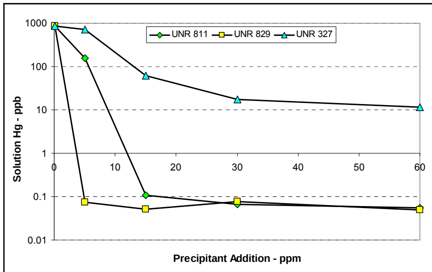
Figure C-10: Mercury Precipitation Tests on Detoxified Leach Tails Slurry
