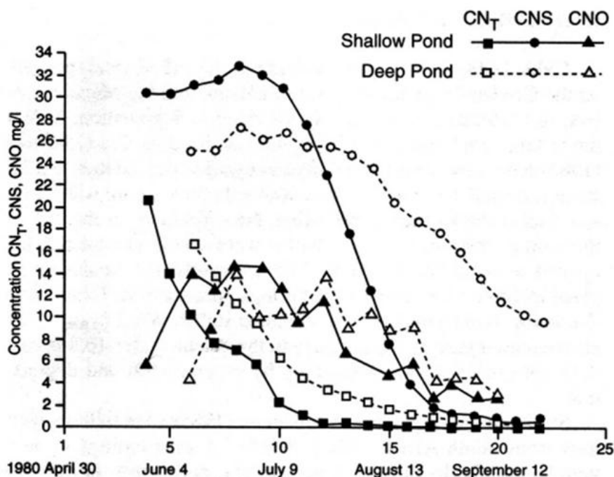
Figure 3: Natural Cyanide Degradation in a Northern Canadian Mine (Meech, 2013, as presented in Hatch, 2015c)
