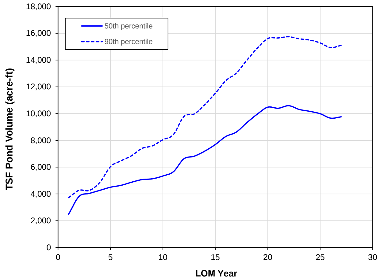
Annual TSF pond volumes over the life-of-mine using the stochastic water balance model.
