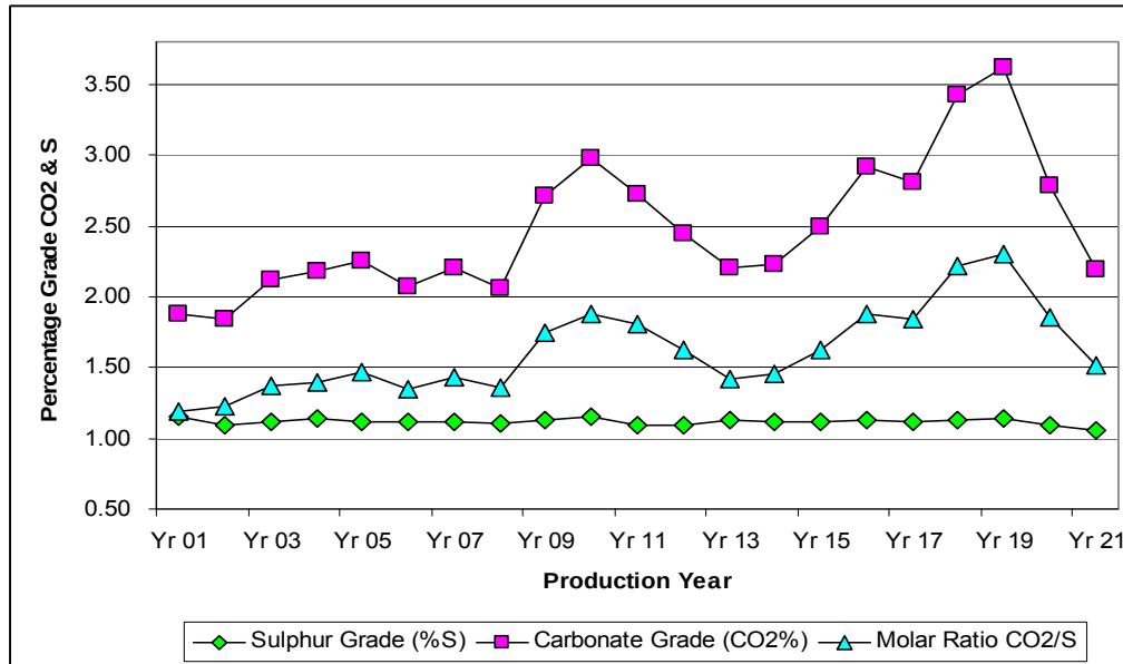
Figure C-7: Production Plan for Sulfur, Carbonate, and Molar Ratio (Carbonate/Sulfur)
