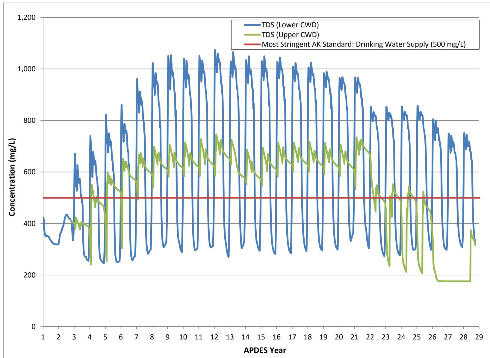
Figure 5: Predicted TDS Concentration in the Upper and Lower CWDs
