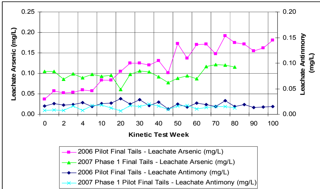
Figure C-5: Kinetic Cell Testing Profiles (As, Sb) of Two Final Tailings Samples
